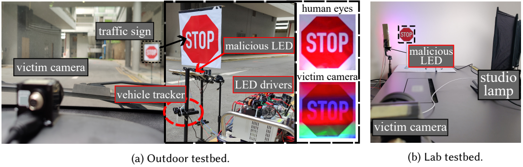
Fig. 7. Testbed setups.
