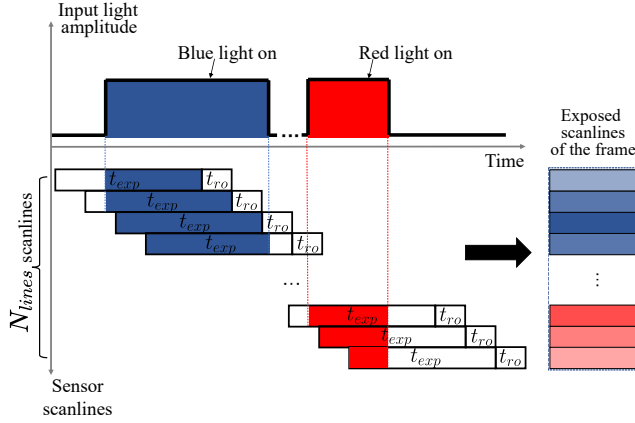
Fig. 2. Rolling shutter's operation and RSE.
