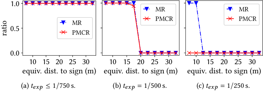
Fig. 17. Effectiveness vs. sign-camera distance under different t_{exp} .
