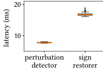
Fig. 25. Latencies of GhostBuster on Jetson Orin.
