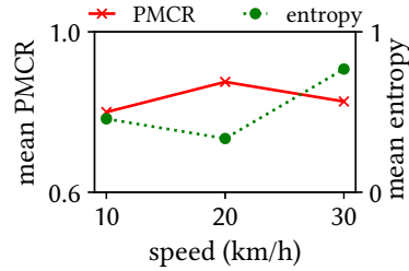
Fig. 13. Impact of victim vehicle's speed.
