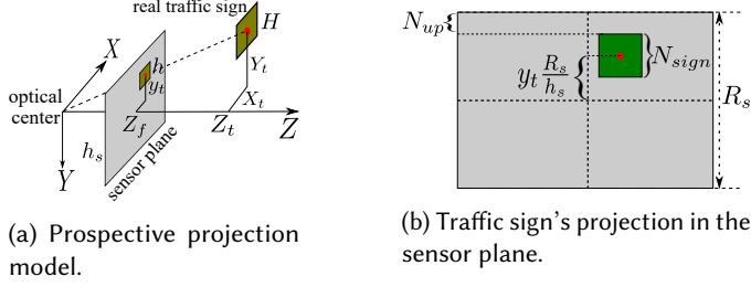
Fig. 5. Estimation of the traffic sign's vertical position and size in the captured image.
