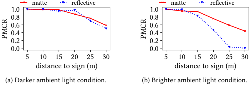
Fig. 15. Impact of traffic sign texture.
