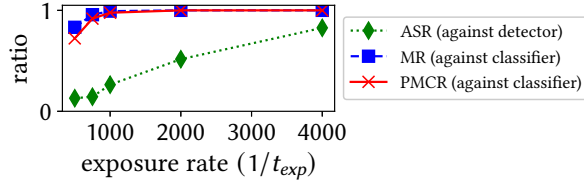
(a) ASR of GS-D under different exposure settings.
