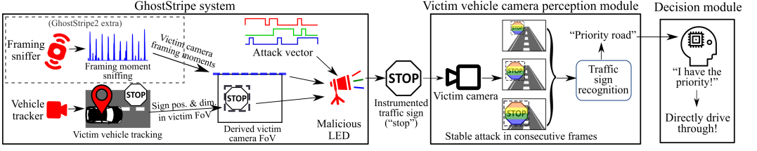
Fig. 4. Overview of GhostStripe.
