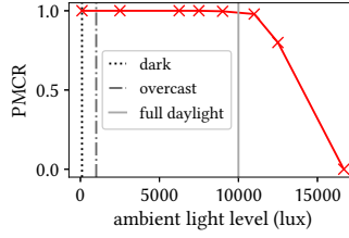
Fig. 19. Effectiveness vs. ambient light.
