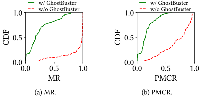
Fig. 24. Comparisons of GhostStripe's effectiveness on real-world trials with and without GhostBuster.
