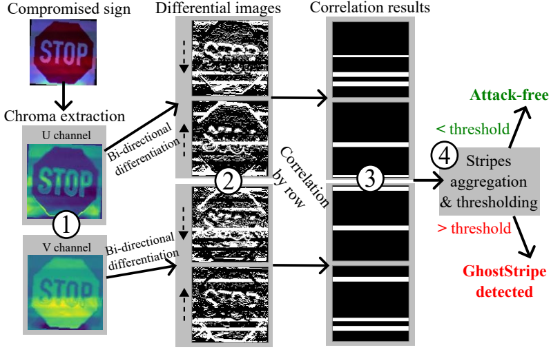
(a) Pattern correlation-based detection against GhostStripe.
