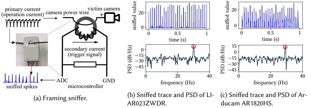
Fig. 6. Framing sniffer and measurement traces.
